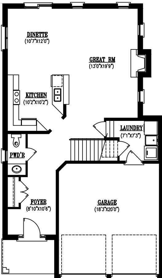
MAIN FLOOR PLAN 915 SQ.FT.
