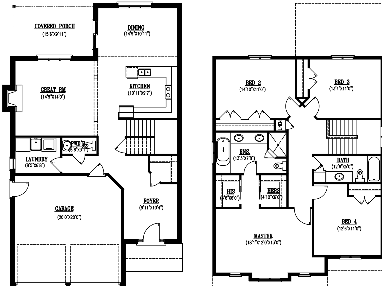
UPPER FLOOR 1287 SQ. FT.
